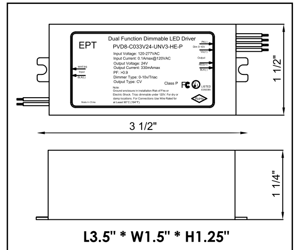
LED DRIVER DIAGRAM
